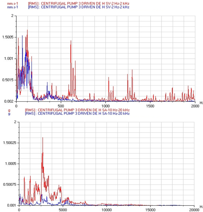
Fig. 5. Vibration amplitude, on the Pump drive end, frequency 0 to 2000Hz& 20000Hz.
