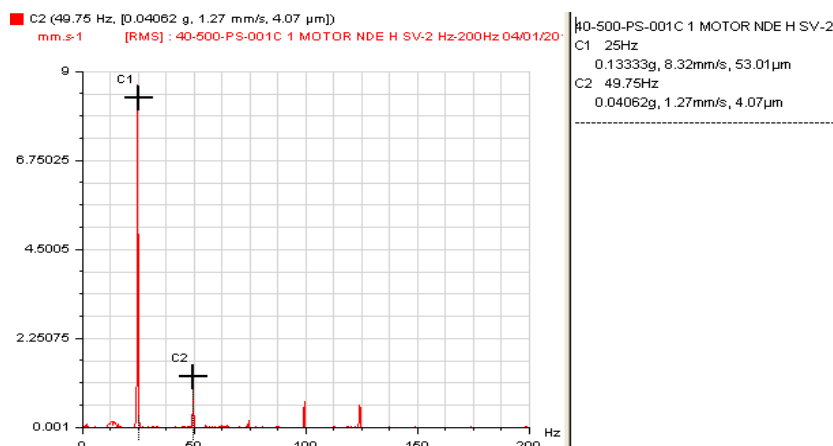
Fig. 19. Trends below show the value of vibration on different points of the Motor and Pump
